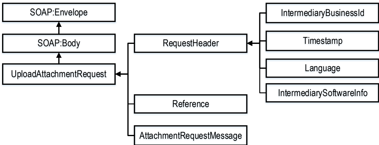
Bild 16: UploadAttachment, begäran
