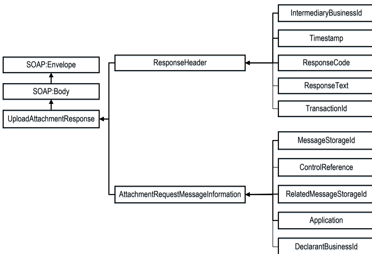
Bild 18: UploadAttachment, svar
